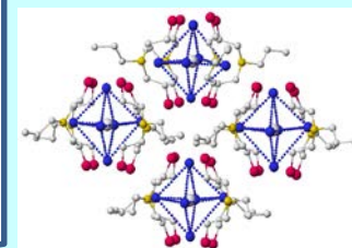
Zero, one - dimensional structure
